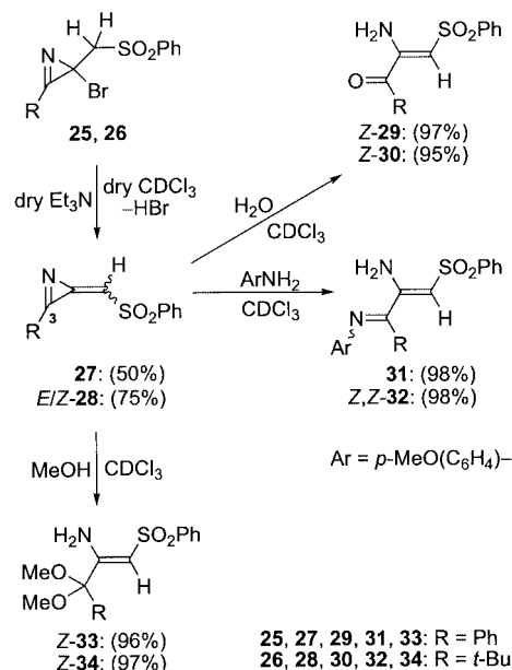
Scheme 5. Generation of methylene-2 H -azirines and subsequent reactions with nucleophiles.
