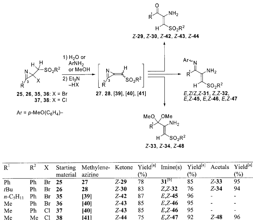
Scheme 6. One-pot synthesis of ketones, imines, and acetals including trapping of methylene-2 H -azirines. [a] Yield of isolated compound. [b] Mixture of isomers.
