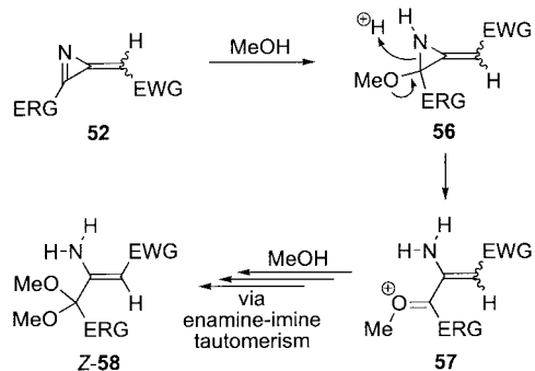
Scheme 9. Mechanism of the reaction of methanol with methylene-2 H -azirines.
