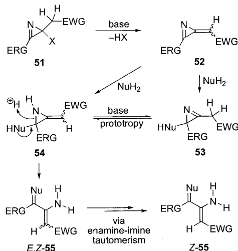
Scheme 8. Mechanism of the reaction of binucleophiles with methylene-2 H -azirines.
